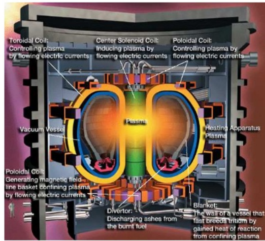
Figure 4 – Construction of the ITER reactor [6]
