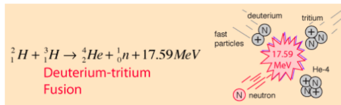
Figure 2 – Nuclear fusion [3]
