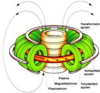
Figure 3 – Tokamak principle [5]
