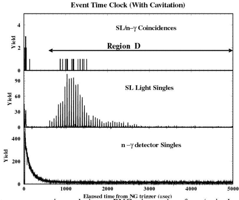
Fig. 2. Event occurrence time relative to PNG trigger time for n^- singles, SL light emission singles, and the SL/ n^- coincidences.
