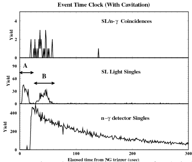
Fig. 3. Event occurrence time relative to PNG trigger time for n^- singles, SL light emission singles, and the SL/ n^- coincidences shown with an expanded time scale.
