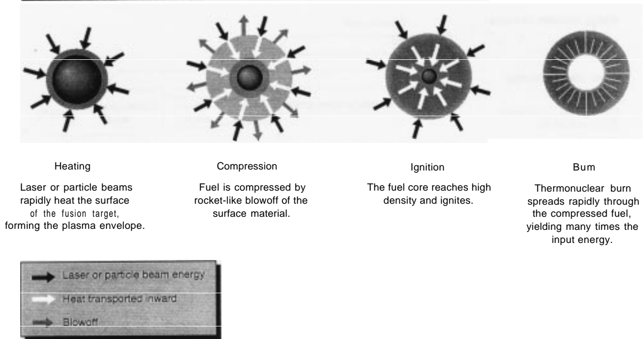
FIGURE 4-1: Inertial Confinement Fusion Process
