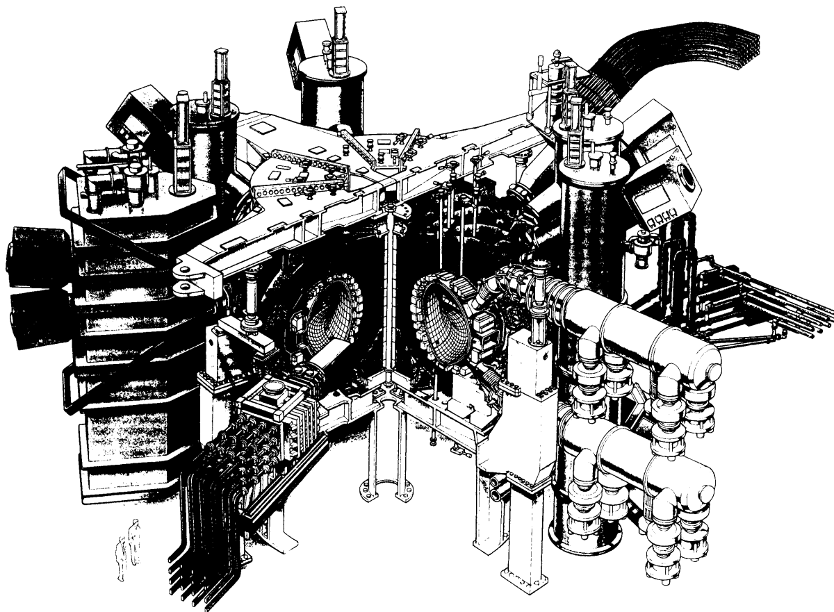
The JT-60U tokamak in Japan.
