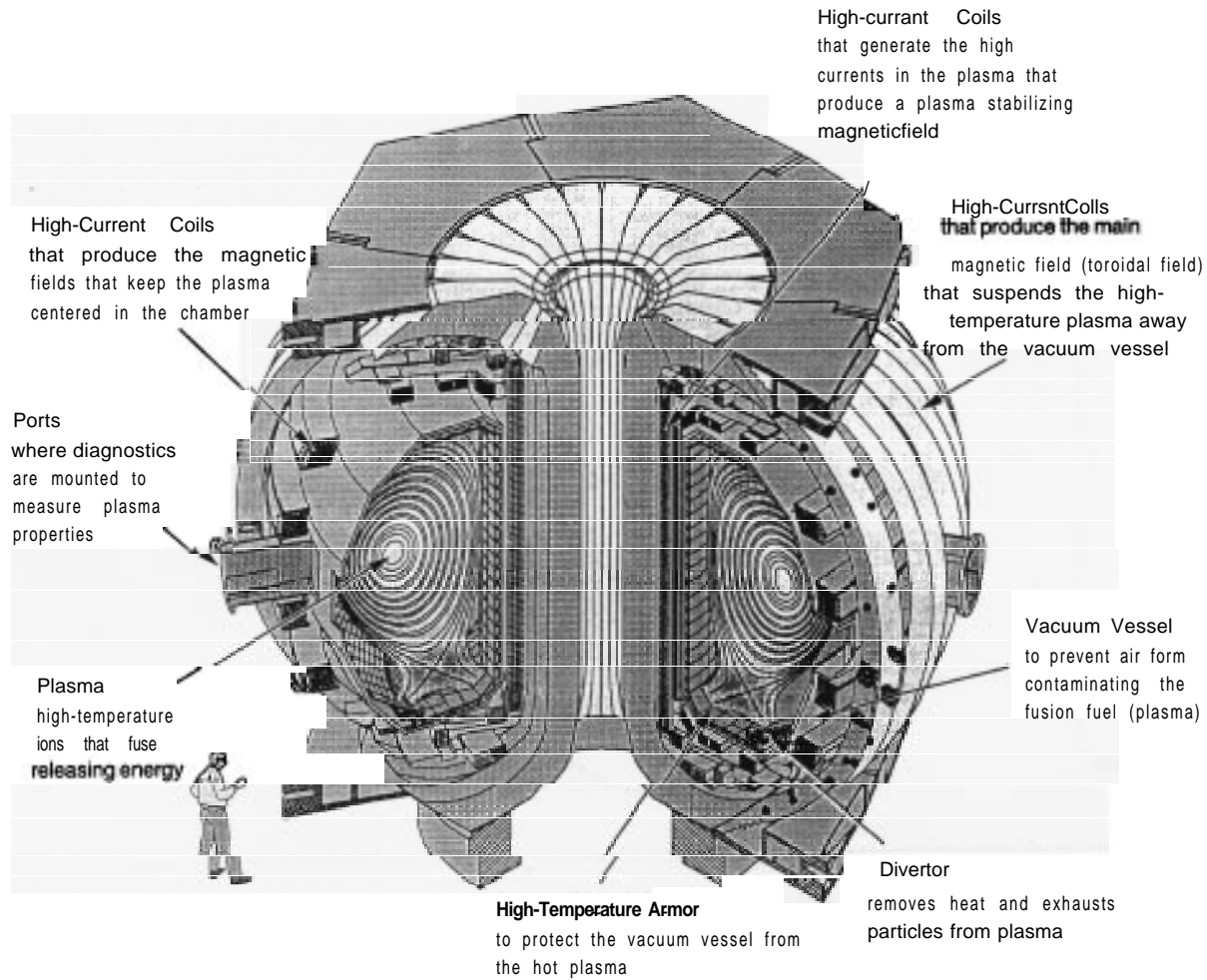
Diagram of General Atomics DIII-D Tokamak showing major components.
