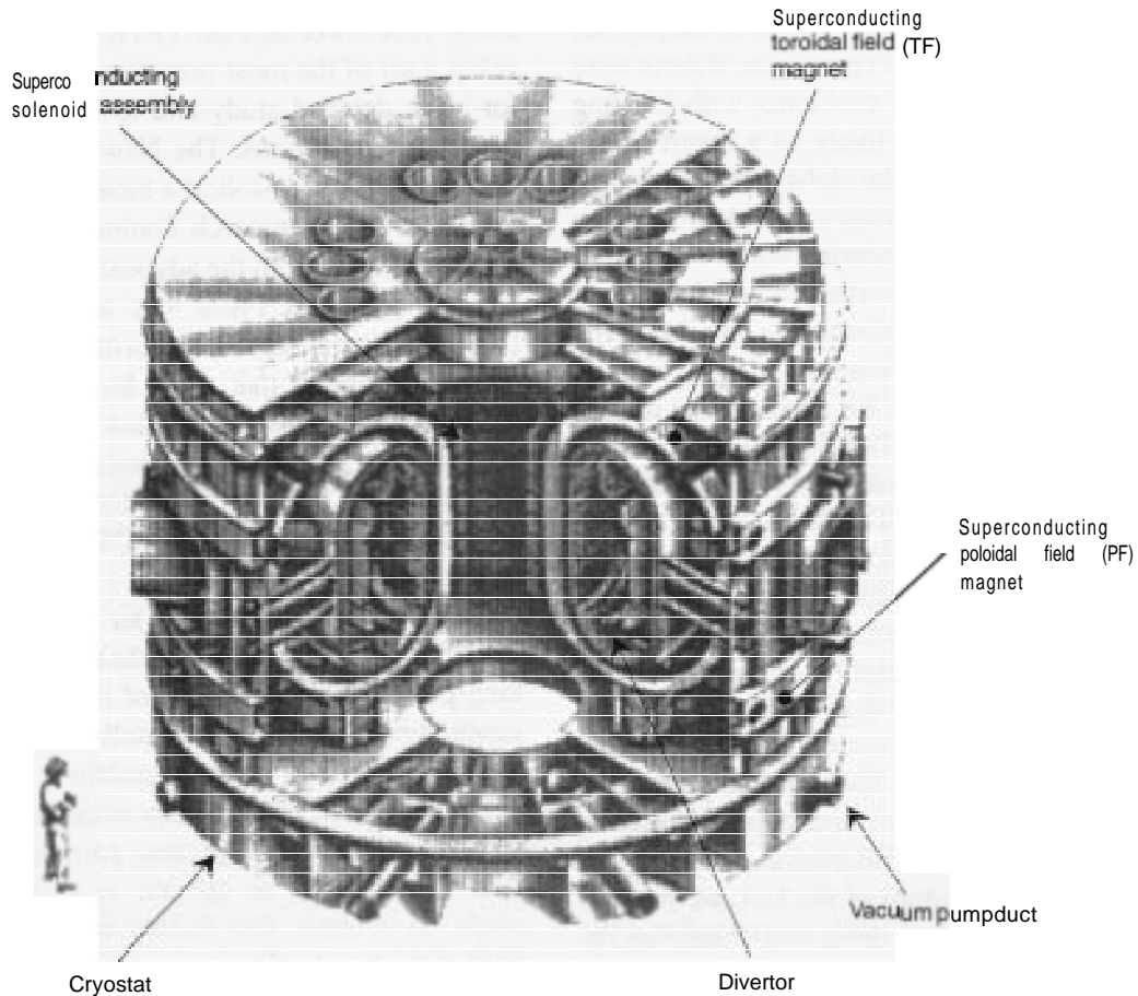
Major TPX components.
