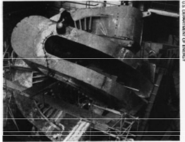
End magnets for the Mirror Fusion Test Facility (MFTF-B) Lawrence Livermore National Laboratory
