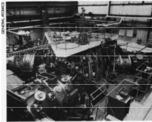
The DIII-D Tokamak at General Atomics in San Diego.
