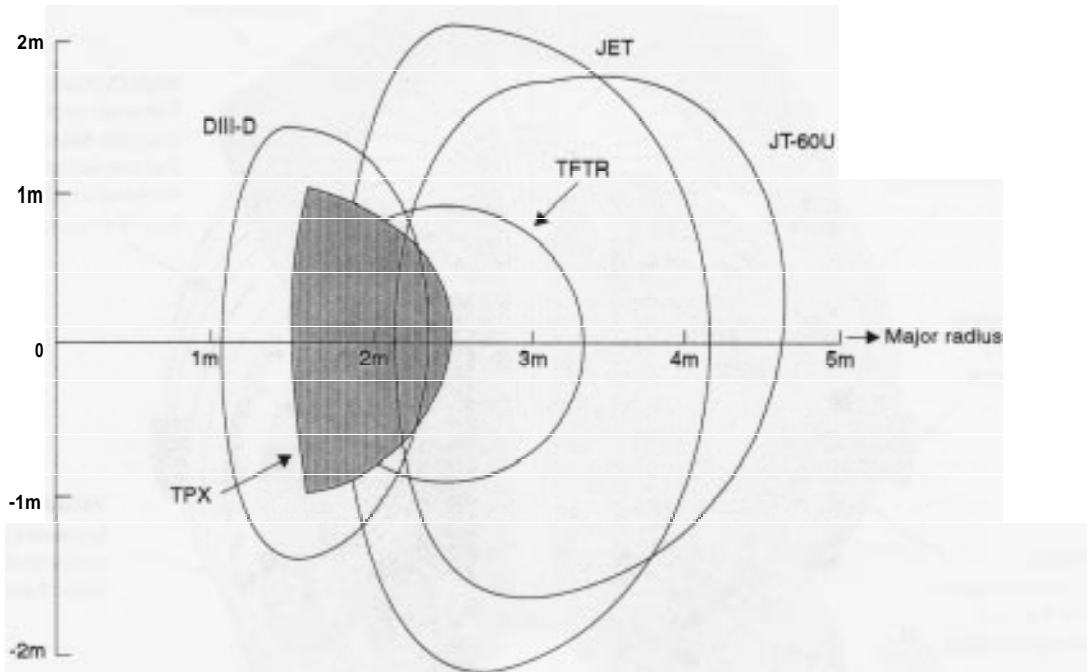
FIGURE 3-2: Comparison of Plasma Cross-Sections of Selected Large Tokamaks
