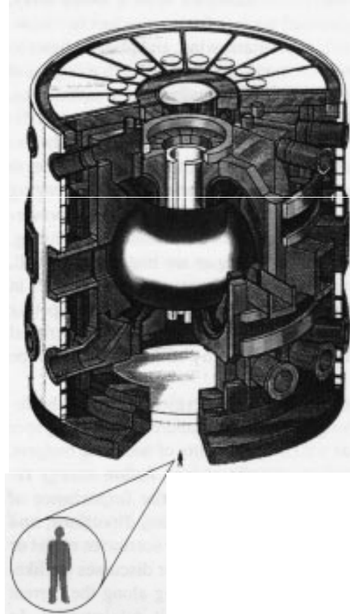
The proposed International Thermonuclear Experimental Reactor.
