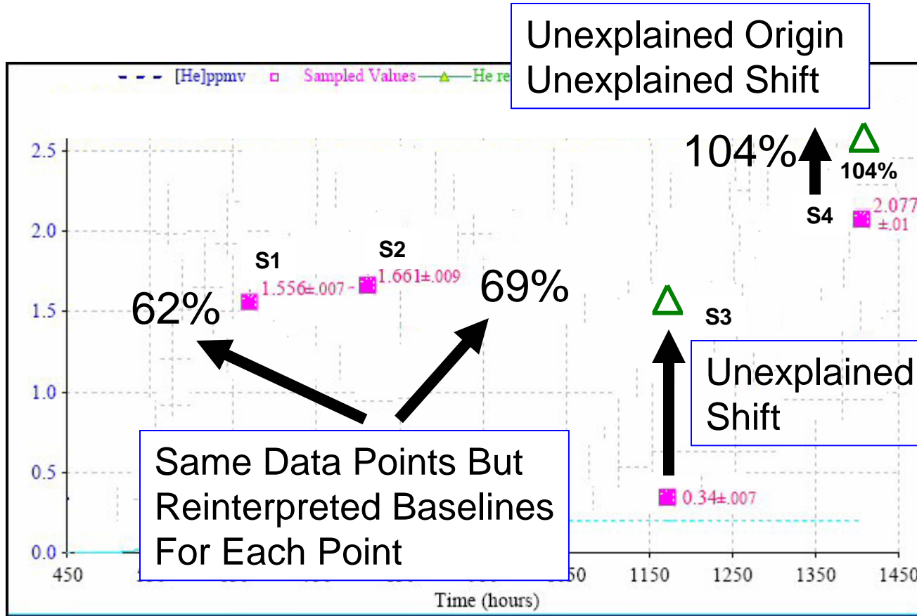
Image from McKubre, ICCF-10, 2003. Bold black arrows and text added by SBK. Green triangle (redrawn) and "104%" (re-written) come from McKubre, ICCF-10, 2003
