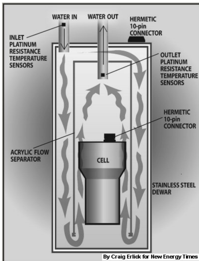
Fig. 3. SRI International-type flow calorimeter.
