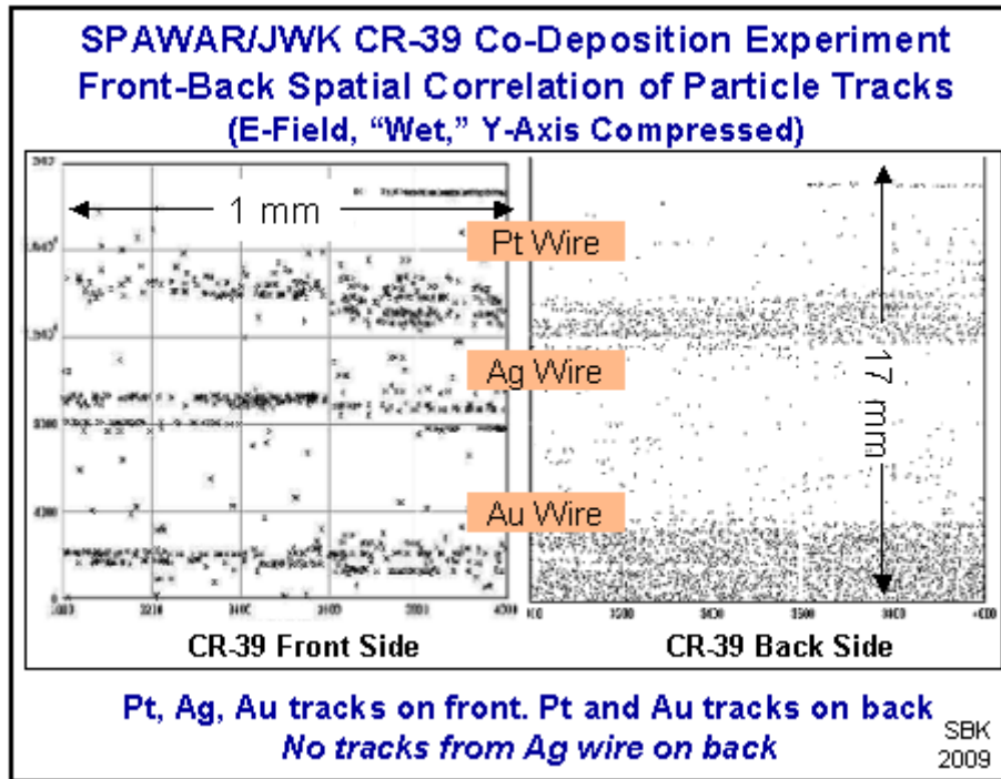
Fig. 11. Front and backside spatial correlation of particle tracks from SPAWAR LENR experiment
