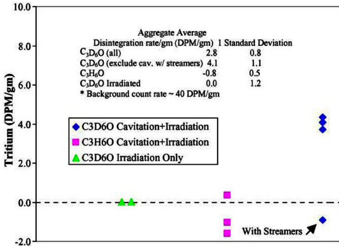
Fig. 23. Three of four experiments showed 4-5 SD signals of tritium from Xu/Butt bubble fusion replication. The fourth experiment displayed "streamers," which indicates that the experiment did not achieve the correct thermohydraulic conditions. 39
