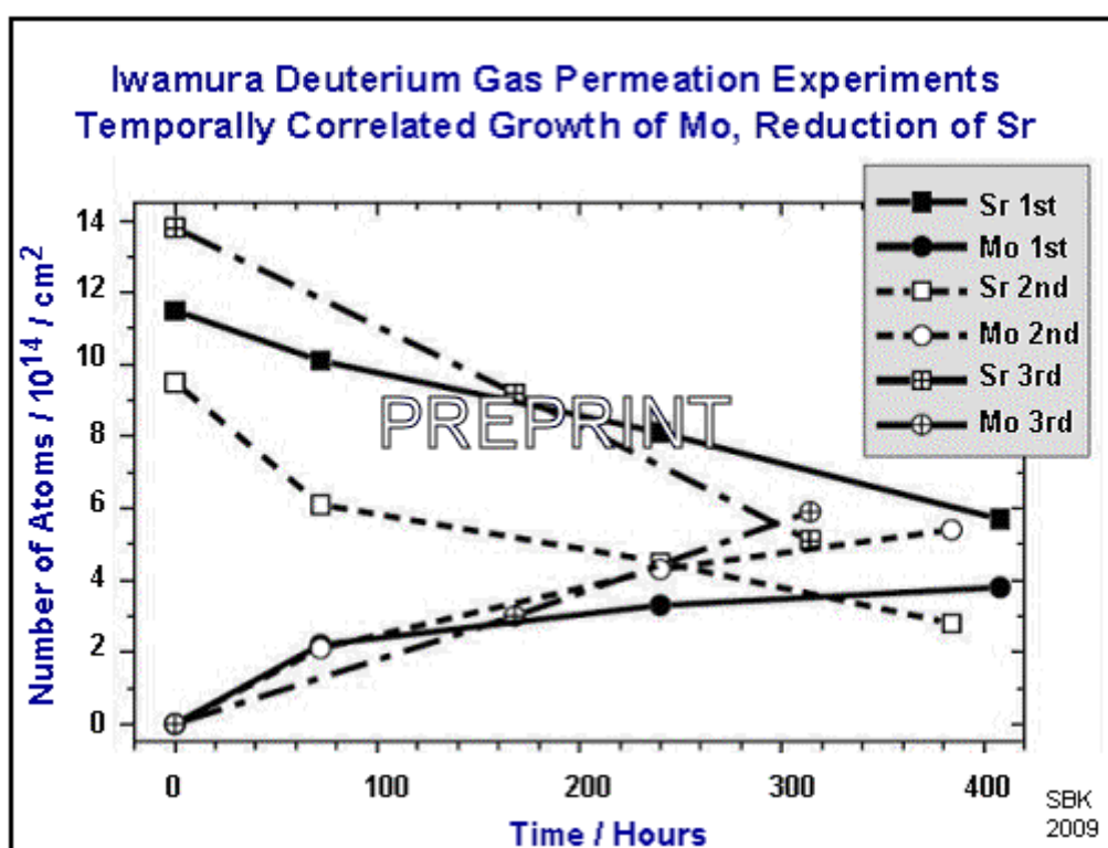
Fig. 16. Three experiments performed by Iwamura and Takehiko Itoh, Mitsubishi Heavy Industries: Increase of Mo and temporally correlated decrease of Sr. 27
