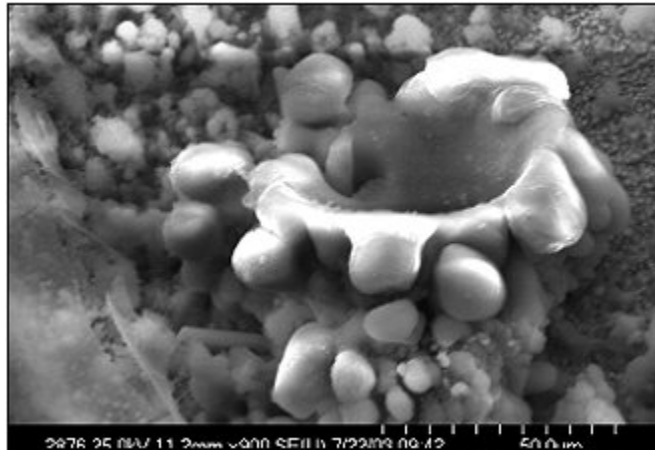
Fig. 7. SEM image of molten Pd on Au foil used as a cathode in a 2003 SPAWAR co-deposition experiment with an external electric field (6000 V). Appears similar to quickly heated molten metal followed by fast cooling from immersion in electrolyte. Photo: Charlie Young. 16
