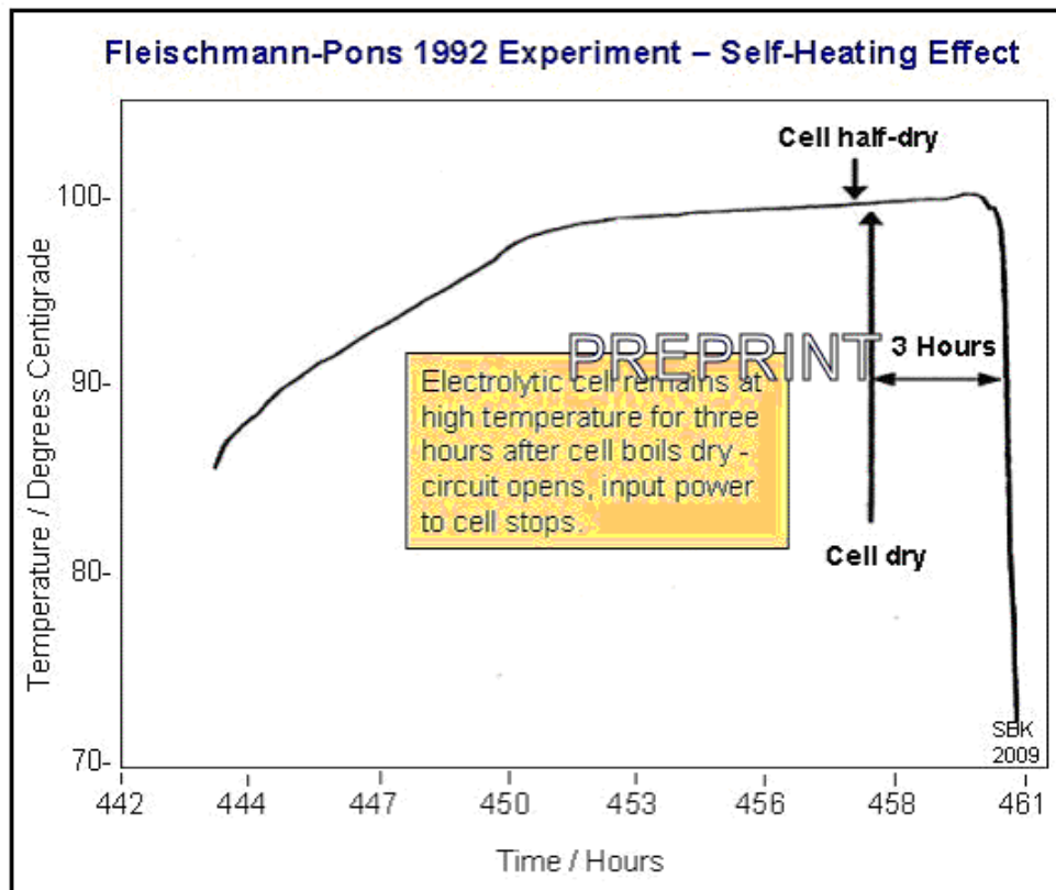
Fig. 4. Fleischmann-Pons 1992 experiment showing self-heating evidence. Image based on Fig. 11 in 1
