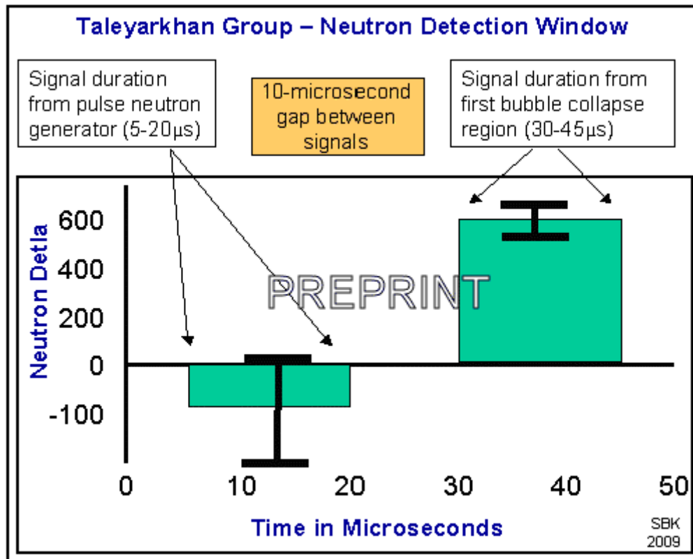
Fig. 22. Time sequence of neutron signals in Taleyarkhan group's bubble fusion experiment. The 10-microsecond gap allowed them to discern neutrons emitted from the pulse neutron generator from the bubble fusion experiment.
