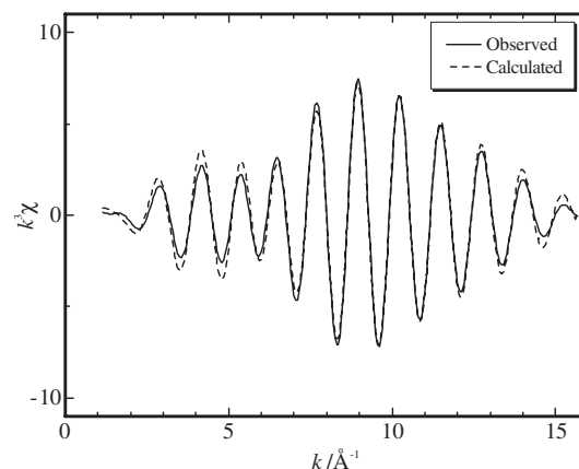
Fig. 4. Representative curve-fitting results using the Pd–Pd one shell model for Vac as an example.
