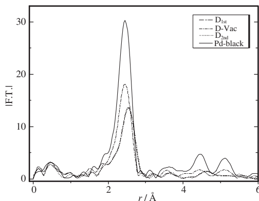
Fig. 3. Radial distribution functions (RDF) for the D 1st , D-Vac, D 2nd and Pd-black nano-sized-Pd/ZrO 2 composites.
