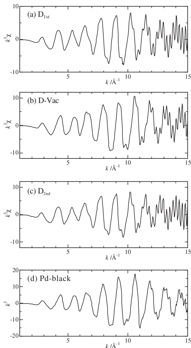
Fig. 1. Pd K-edge EXAFS oscillation function k^3\chi(k) for (a) D 1st , (b) D-Vac, (c) D 2nd and (d) Pd-black.
