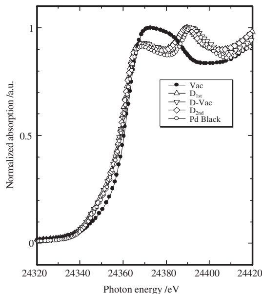
Fig. 2. XANES spectra of Pd K-edge for the D 1st , D-Vac, D 2nd and Pd-black nano-sized-Pd/ZrO 2 composites.
