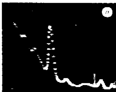
FIG. 1 a, The \gamma -ray background spectrum measured with a 3 in. \times 3 in. NaI(Tl) detector at MIT. Some important terrestrial \gamma -ray lines have been identified in this figure 5,7,12 . (As explained in ref. 12, the immediate parent of the final decay product is identified. For example, 40 K [ \beta^- ] decays into an excited nuclear state of 40 Ar, which actually then emits the 1.460-MeV photon discussed in the text.) The spectrum is averaged over an 84-hour run. b, The \gamma -ray spectrum shown on television by Fleischmann et al. The main characteristics of the two spectra are similar; one can also tell that the two detectors have comparable spectral resolution. In b, note the curious structure at about 2.5 MeV and that beyond the 208 Tl peak (2.61 MeV), which appear to be artefacts. (The spectrum can also be obtained from KSL-TV in Utah (M. Hawkins, personal communication).)
