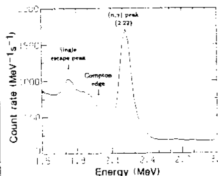
FIG. 3 The \gamma -ray spectrum measured by a 3in. \times 3in. NaI(Tl) spectrometer during a neutron-capture-by-hydrogen experiment using a (Pu/Be) neutron source submerged in water. Because of the finite size of the crystal (which is identical to that of Fleischmann et al. 3 ), we also see an escape peak 2,4 and, of particular importance here, the Compton edge 4 . In this figure, the digitization energy width is 0.024 MeV per channel. The full Pu/Be and background spectra are shown in Fig. 4 of ref. 5.
