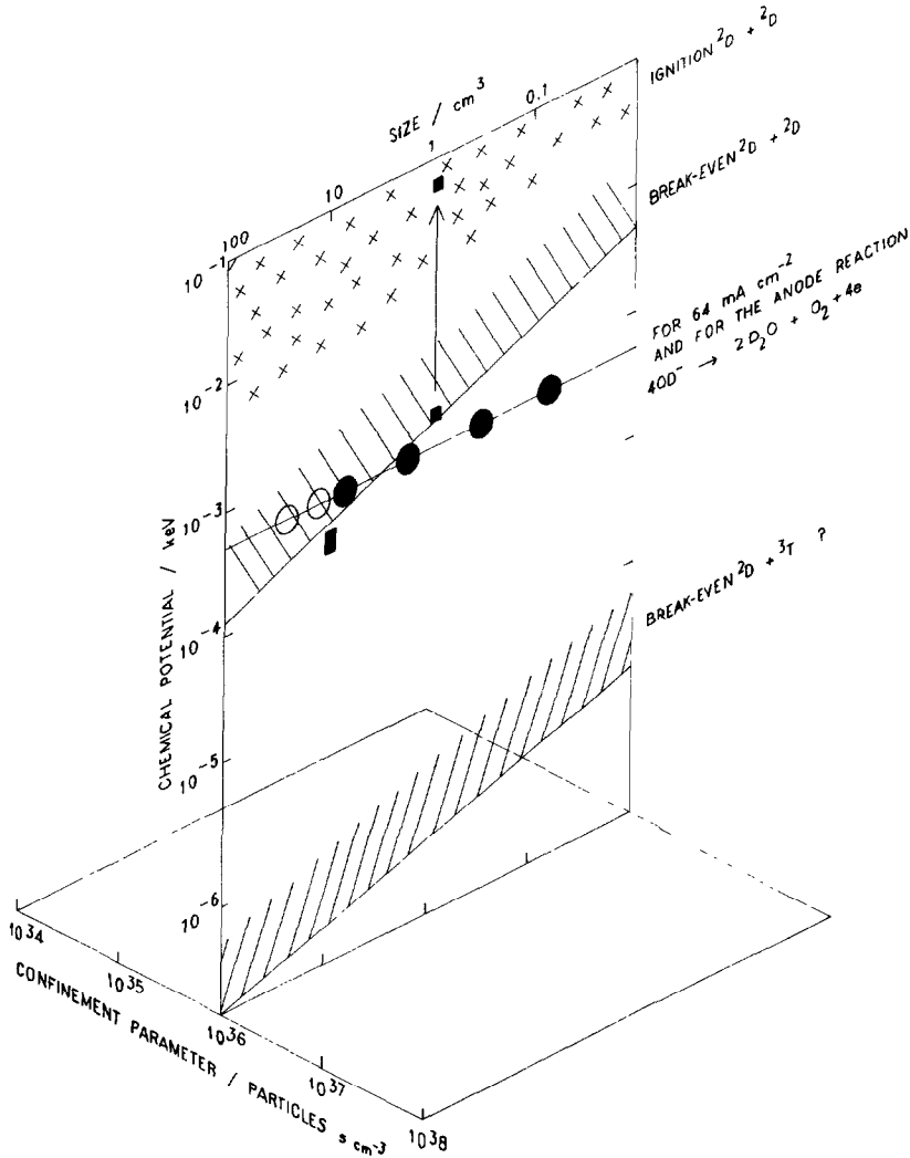
Fig. 2. Confinement parameter–chemical potential–size diagram for {}^2\text{D} + {}^2\text{D} fusion reaction in Pd cathodes; projection to the {}^2\text{D} + {}^3\text{T} reaction. Open circles: systems currently being investigated.
