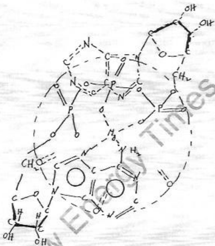
Figure 5. Planar view of two molecules of Mg chelated ATP one directly above the other facing each other. The dashed-line structure represents the lower molecule. The Mg^{++} is at the center of a circle with six dipoles spaced evenly around the circumference - three per molecule of ATP. The adenine part of the adenosine triphosphate straddles the perimeter.
