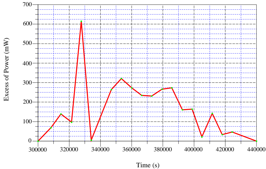
Excess of Power Experiment C1
