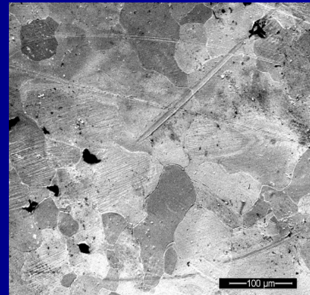
Cold worked and annealed at 850 °C for 1 hr.
