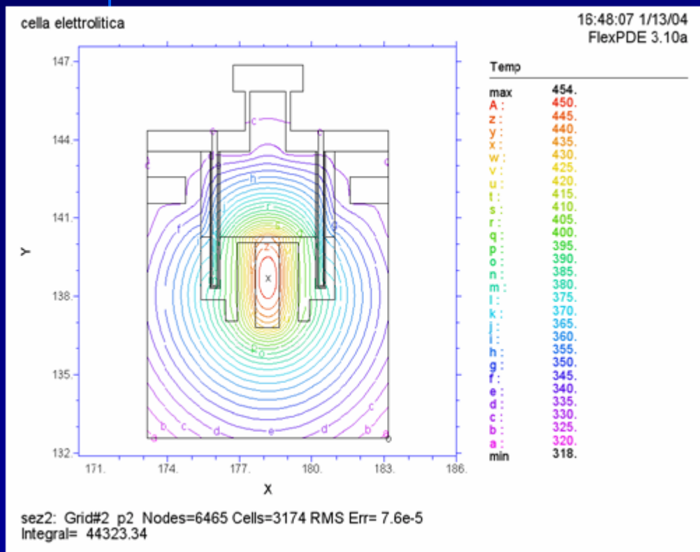
Simulated cell and experimental cell (closed cell with recombiner)
