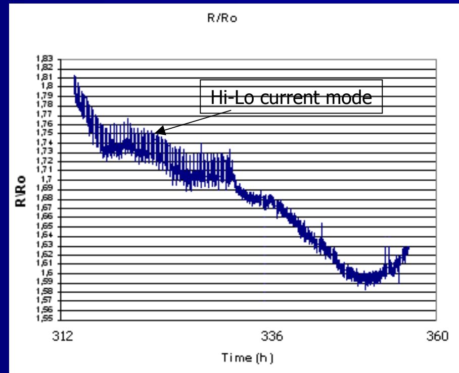
Loading evolution into a treated Pd sample.
