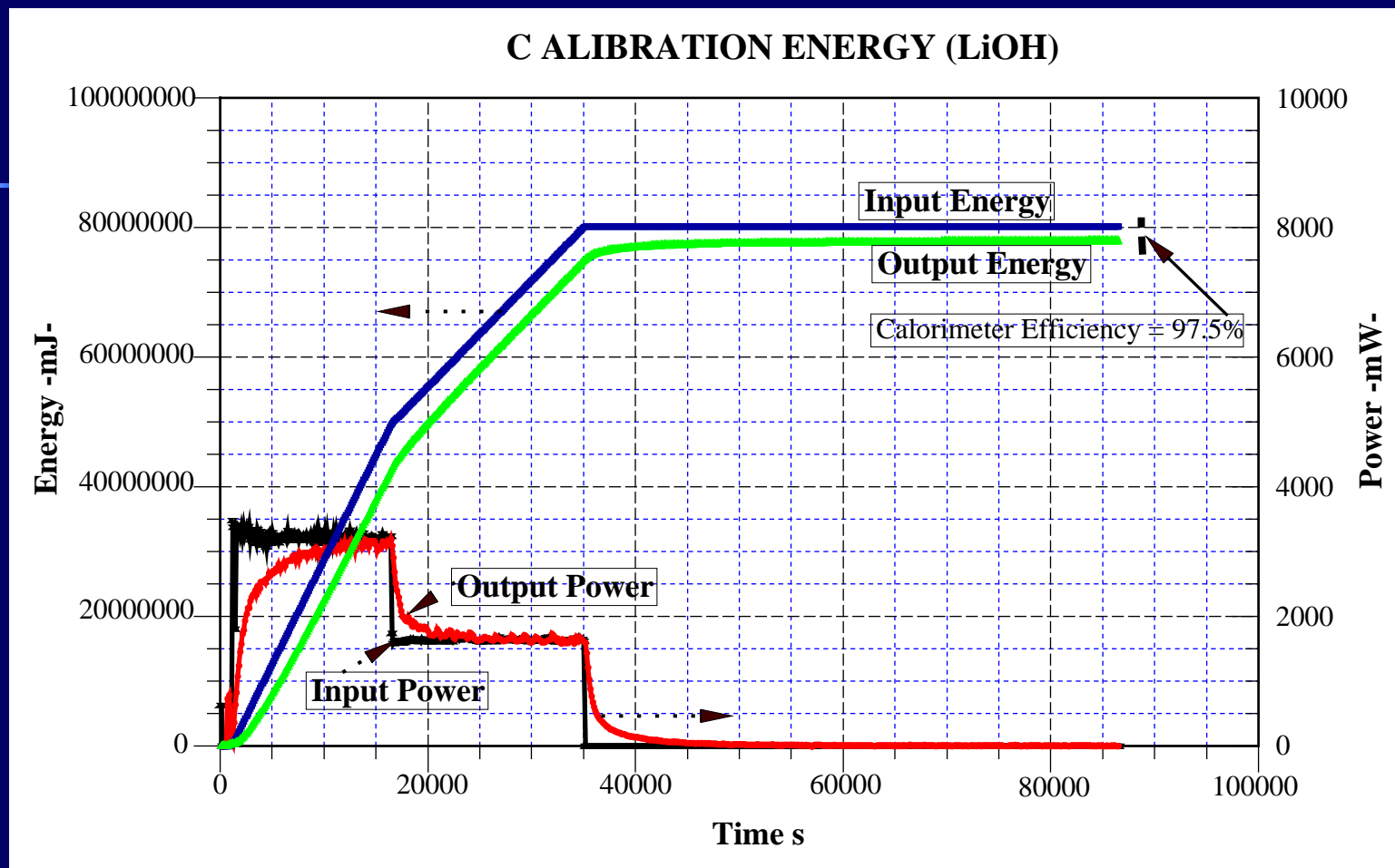
Plot of energy & power (input and output) for calibration with H 2 O 0.1 M LiOH.
