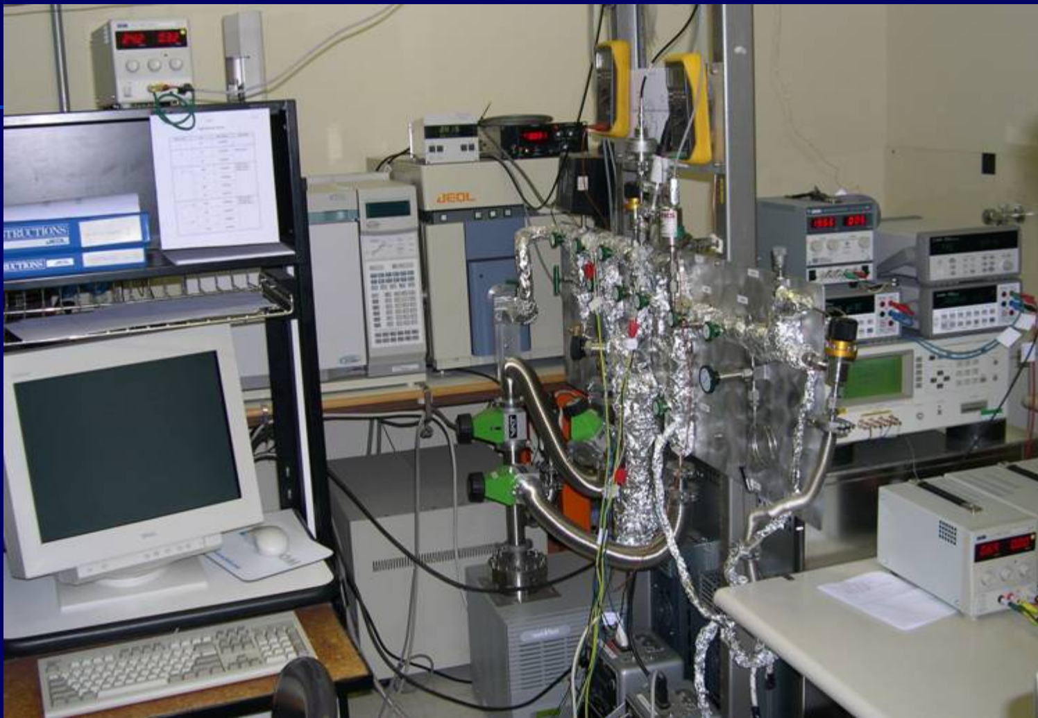
JEOL mass spectrometer and inlet system.
