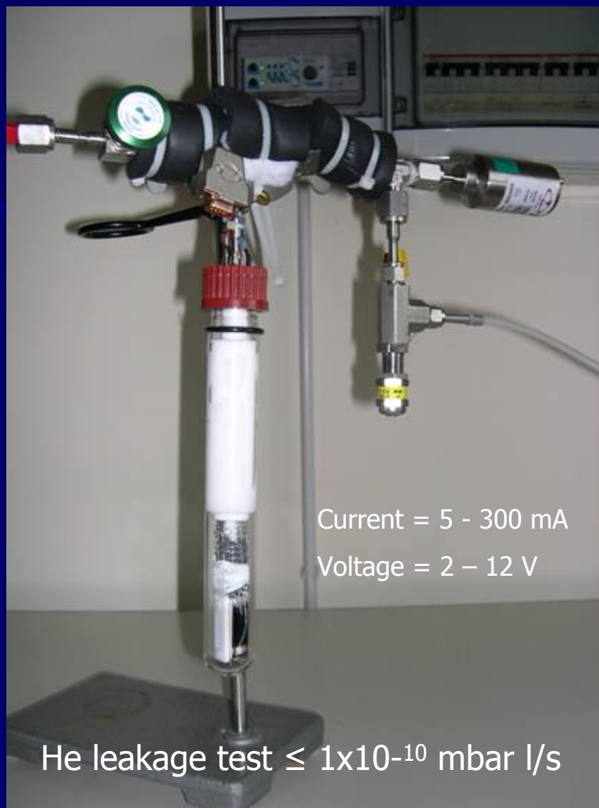
Symmetric electrochemical cell :Pt-foil/Pd-foil/Pt-foil (20x10mmx50 \mu m Pd).
