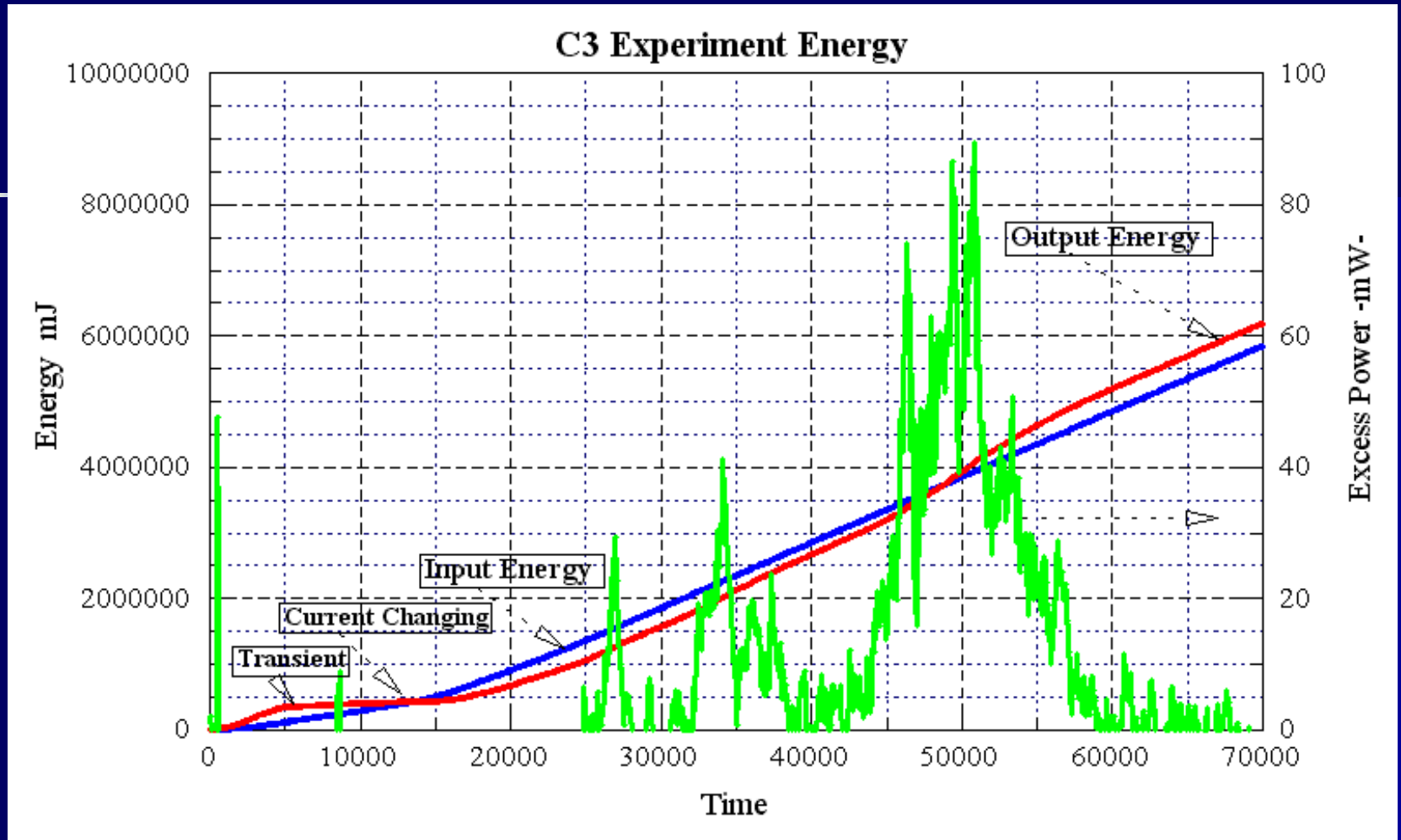
C3 experiment: plot of energy & power (input and output)
