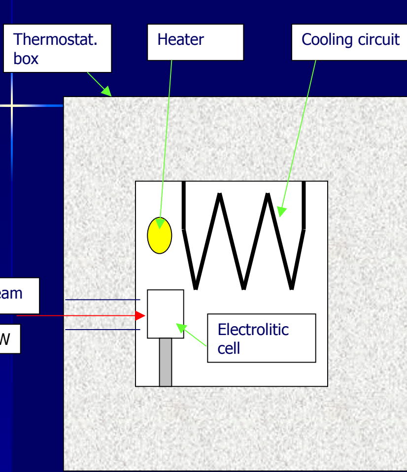
Calorimetric system for laser triggering experiments (T Box = Set p. \pm 0.15 °C)
